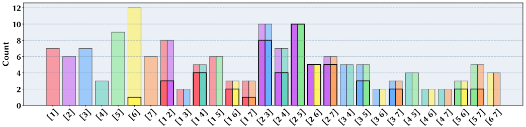
Fig. 13. This picture illustrates the count of policies with a similar configuration of interpolation coefficients among the 150 sampled policies, with the thick line representing the proportion of failed policies. The first group are perturbed policies, and the second one with two bars are perturbed mixes of dances. These groups are described by the sampling criteria in section 5.2. Here, the numbers indicate which of the failing policies Dances 1-7 are prevalent in the mix.
