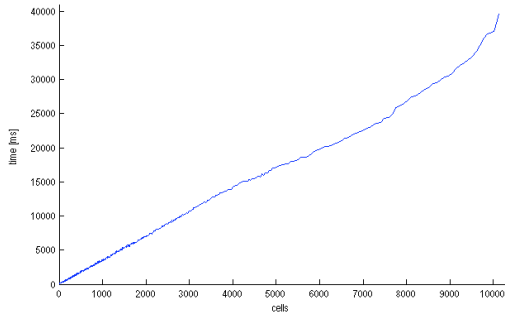
Figure 5: Time performance plot for a foam network evolving over time. The initial number of cells is 10k with a frame time of 39.5s. The last frame contains 11 cells and took 84ms. The simulation ran on a standard single core 2GHz laptop.
