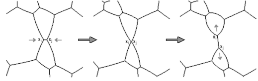
Figure 1: The T1 process on a 2D dry foam. An approaching unstable four-fold vertex will be split into two stable three-fold vertices.
