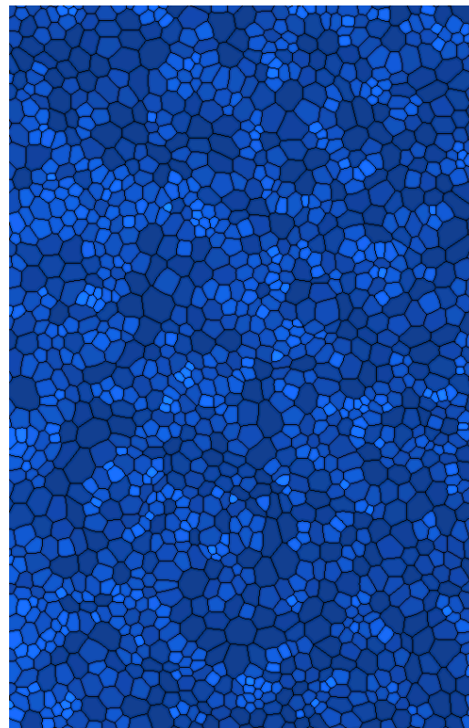
Figure 8: The cell pressures are visualized in flat shaded blue tones. The colors have been exaggerated to make the difference more visible.
