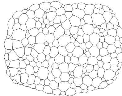
Figure 6: A foam is evolving with initially 10,000 cells. The time step is squared between each shown frame.
