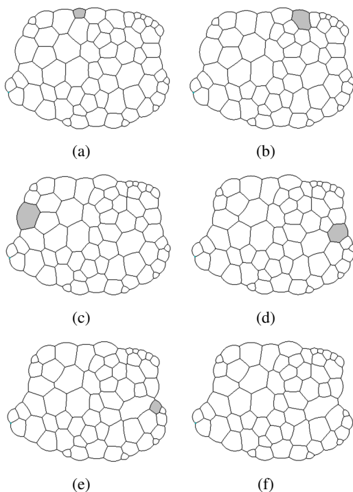
Figure 7: Forced bubble collapse is performed on the dynamic foam boundary. Between each sub figure the marked cell is next to be collapsed.
