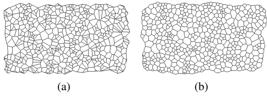
Figure 4: In (a) a Voronoi diagram of 500 cells is generated from random point sites and (b) shows the corresponding equilibrated 2D dry foam network with an area error of 0.001% and an angle error 0.01%.
