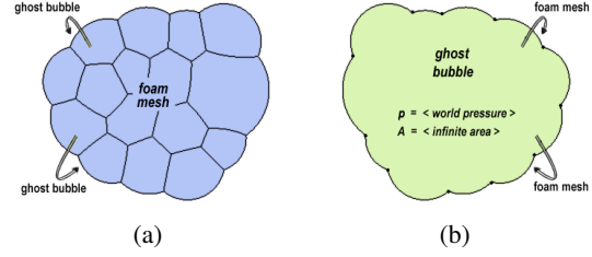
Figure 3: The ghost bubble. (a) The front of the foam mesh defines the foam network. (b) The ghost bubble is defined on the back of the foam mesh where it reuses all existing boundary vertices of the foam. It acts as a mirrored bubble that contains all bubbles in the foam network.
